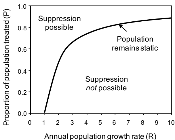
Figure 4. Relationship between MPB's annual population growth rate (R) and the proportion of the population (P) that must be treated for control to suppress population growth. The curve ( P=1-1/R ) represents a static population. Suppression is possible above the curve but is not possible below the curve. Adapted and redrawn from Carroll et al. 2006.
