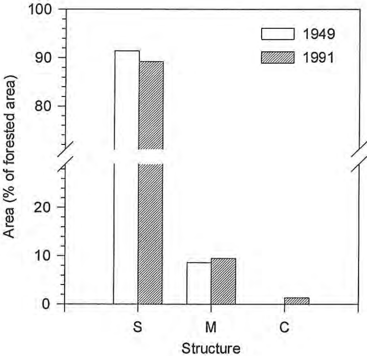
Figure 3-4: Stand structure within coniferous forest in 1949 and 1991 (expressed as % of forested area). S – single canopy, M – multiple canopy, C – complex canopy structure.
