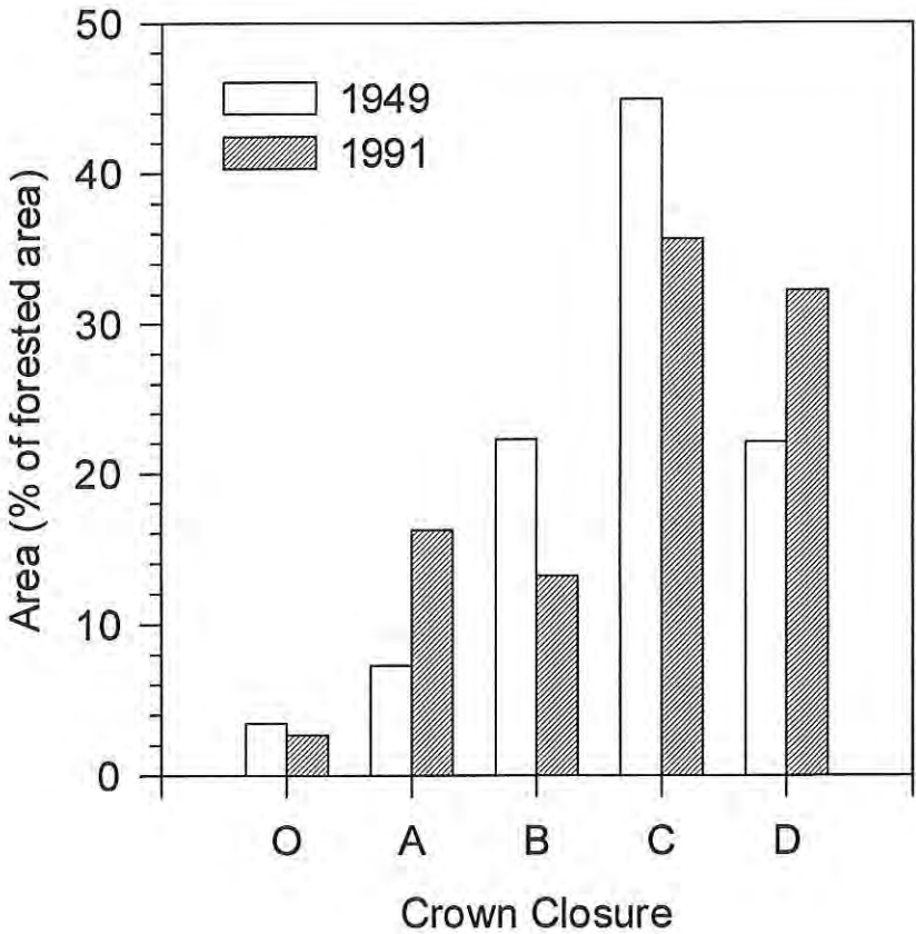
Figure 3-6: Change in crown closure, 1949 to 1991, within coniferous forest (expressed as % of forested area). O – 6-15% cover, A – 16-30%, B – 31-50%, C – 51-70%, D – 71-100%.
