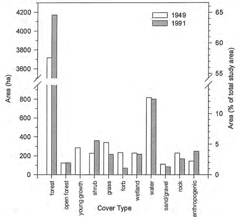
Figure 3-2: Landscape cover in percent area and absolute area (ha) in 1949 and 1991 by cover class.
