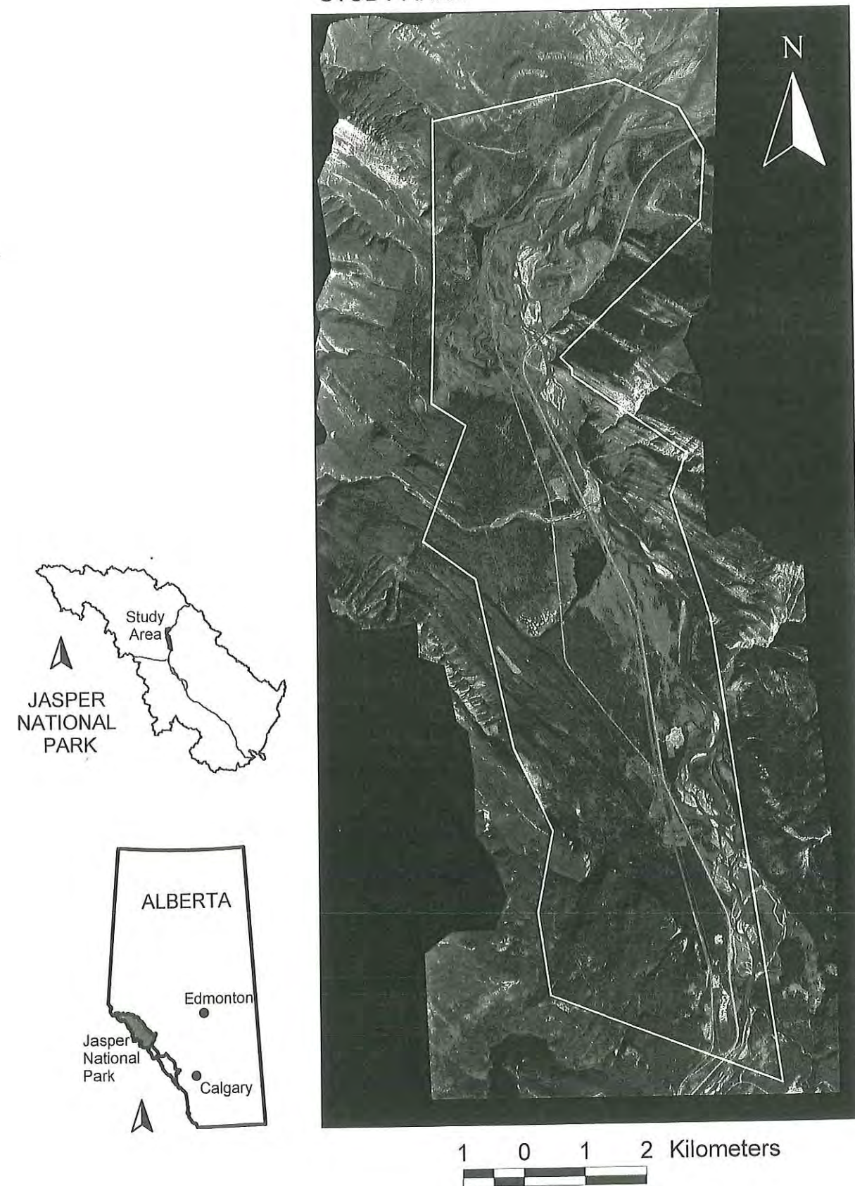
Figure 2 - 1: Study Area. White line represents the boundary of the study area in the montane ecoregion in the central area of Jasper National Park, Alberta.
