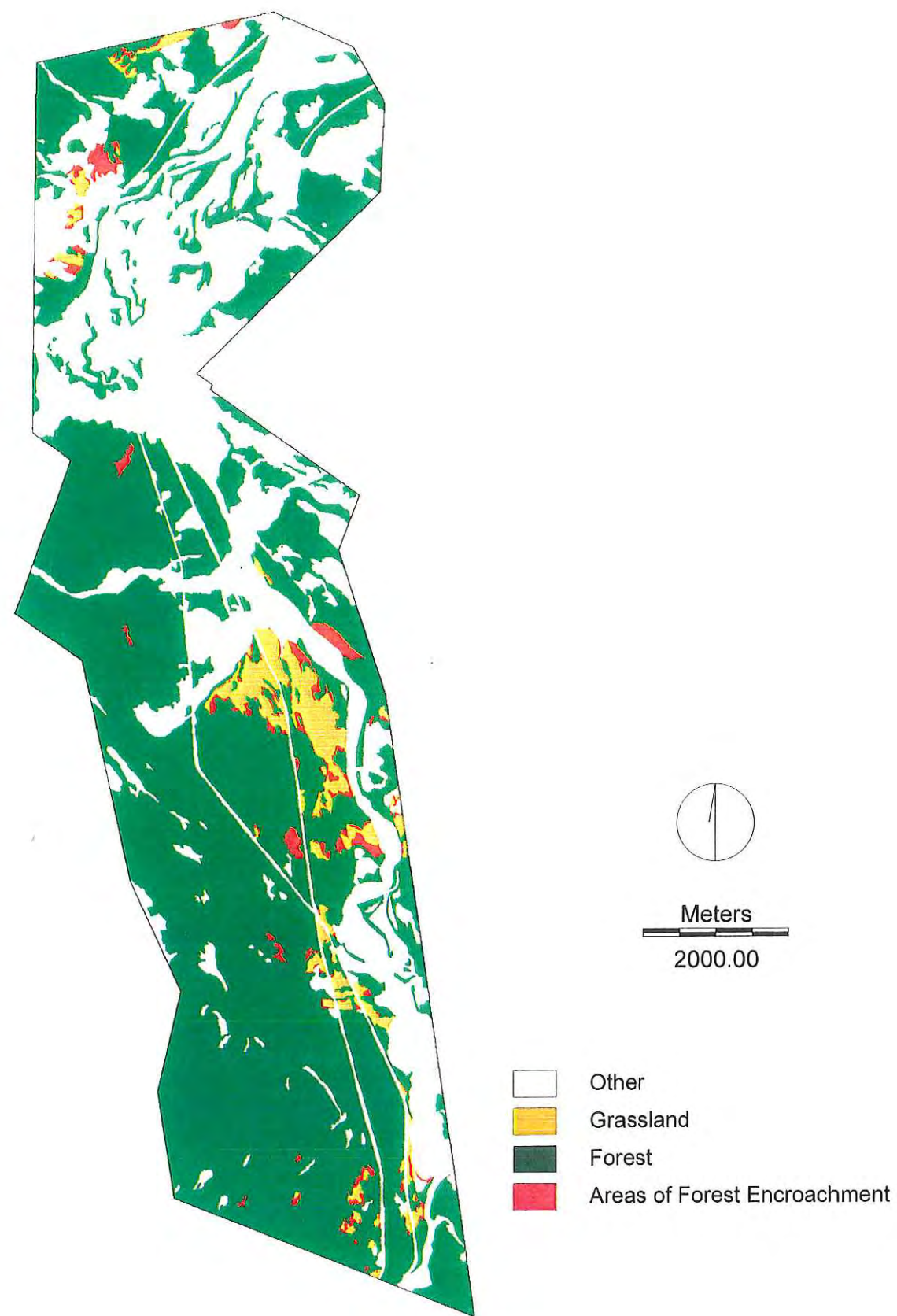
Figure 3-8: Forest Encroachment onto Grasslands, 1949 to 1991
