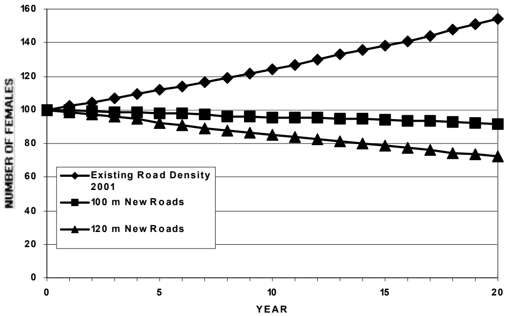
Fig. 4.1. Expected population change for the ALP herd based on different densities of new roads within a woodland caribou MCP.
