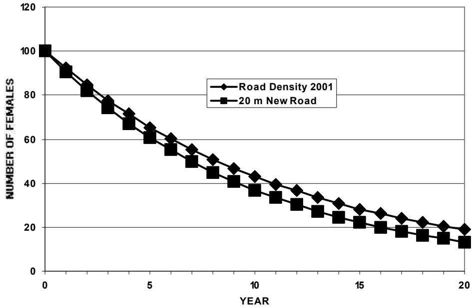
Fig. 4.3. Expected population change for the LSM herd based on different densities of new roads within a woodland caribou MCP.
