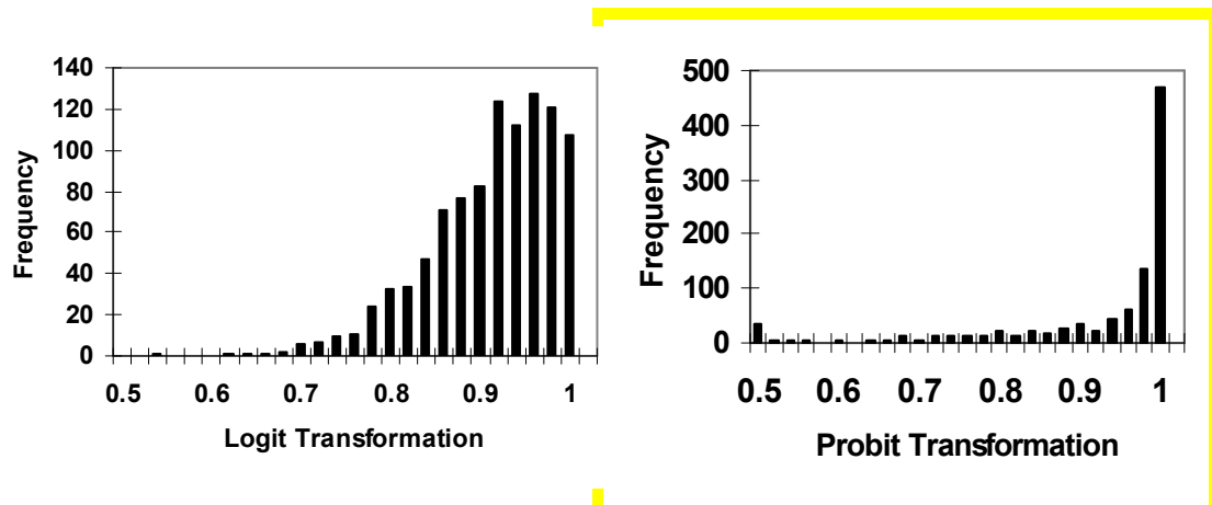
Fig. 2.7. Histograms comparing the inverse log-normal distribution (logit transformation) versus the cumulative distribution (probit transformation) of 1,000 randomly generated adult female survival rates based on a mean of 0.912.
