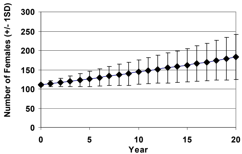
Fig. 2.5. Trajectories of population size projected over 20 years repeated 200 times (a) and the mean ( \pm 1 standard deviation) from 1000 simulation runs (b) of a stochastic model of the A La Pêche woodland caribou herd based on a starting population of 111 females, mean adult survival of 0.907 (SD = 0.069), a mean calf/cow ratio of 0.238 (SD = 0.092) and an assumed calf sex ratio of 50:50. The calf/cow ratio is discounted by 15% to represent over winter mortality of calves. These projections assume no density dependence.
