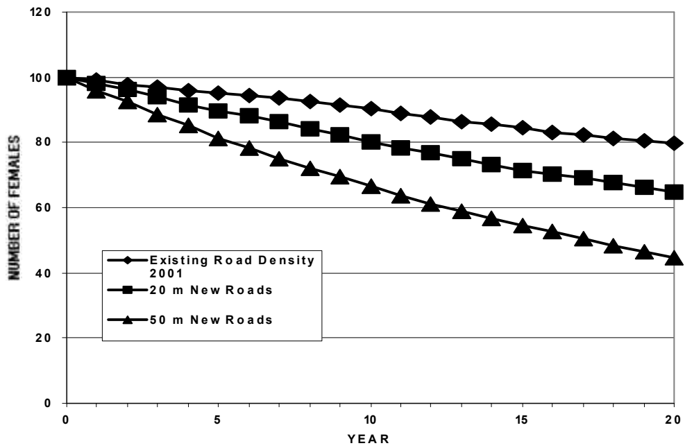
Fig. 4.2. Expected population change for the RPC herd based on different densities of new roads within a woodland caribou MCP.
