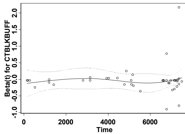
Fig. 3.6. Scaled Schoenfeld residuals vs time of study for beta coefficients of road density, all linear features and cutblocks within 3875 m buffers around woodland caribou locations.
