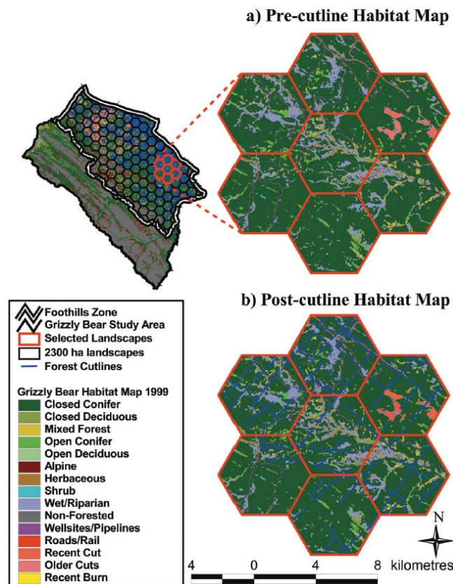
Figure 6. Selected sample of real landscapes showing (a) pre-cutline and (b) post-cutline representations of the grizzly bear land-cover map. Figure from Linke et al. 2008, p. 27.
