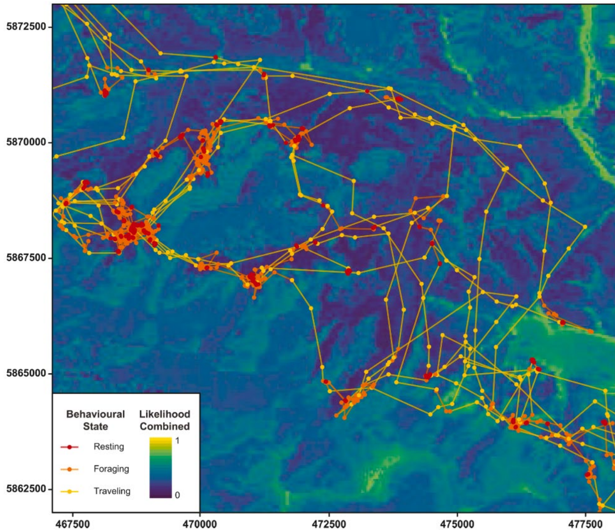
Figure 12. Example of movement states for a grizzly bear overlaying a recreation and tourism likelihood layer. Figure from Goodbody et al. 2021, p. 108.
