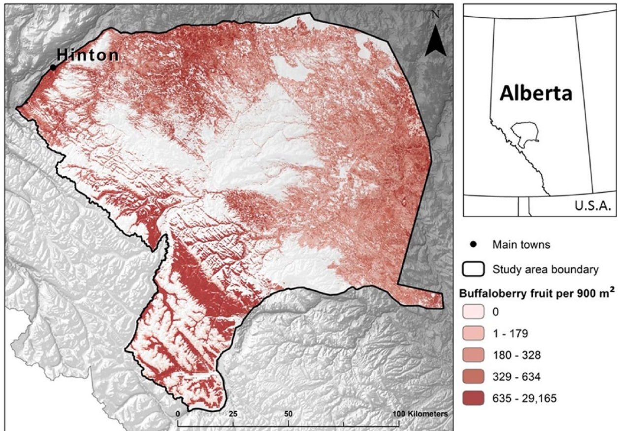
Figure 15. Location of the study area near Hinton, Alberta, Canada defined by a buffaloberry fruit density model (fruit/900 m 2 ) by Nielsen et al. (2017). Fruit density is symbolized based on quantile classification. Figure from Denny et al. 2018, p. 80.
