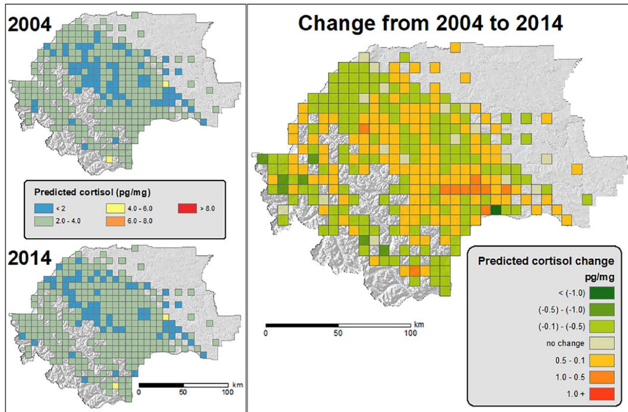
Figure 12. Predicted hair cortisol concentrations in 2004 and 2014 and over time from landscape variables in the most supported model (anthropogenic disturbance and food resource availability). Only this model was supported ( \Delta AIC_c = 0.00 ) when year was included in the final candidate models; however, predicted hair cortisol concentrations were generated from the final model without year. Therefore, unidentified change associated with sample year is likely present. Figure from Wilson et al. 2020, p. 64.
