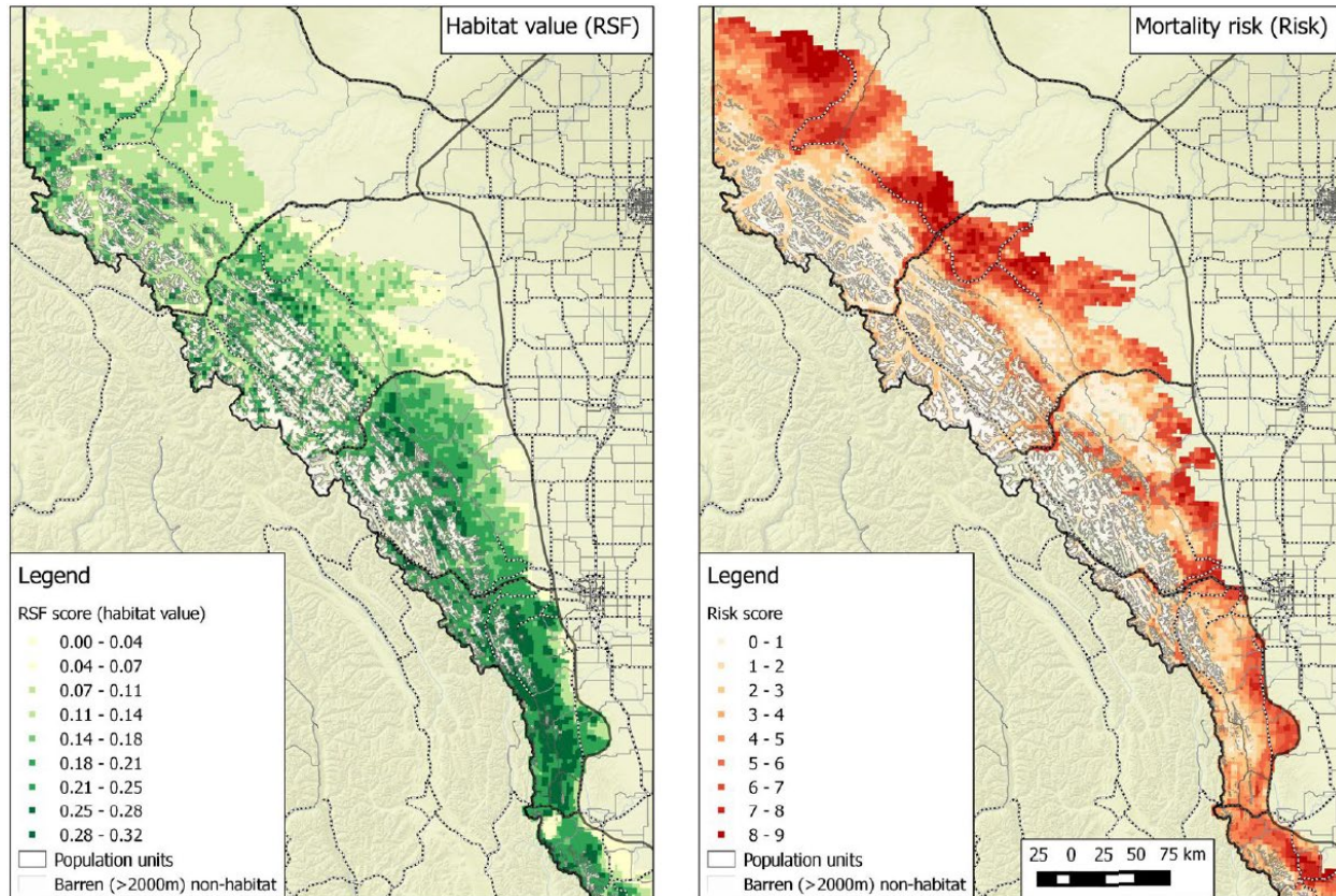
Figure 18. Resource selection function (RSF) scores for grizzly bear habitat (left graph) and mortality risk scores (right graph) used as mark point covariates in the density surface model for analysis of Alberta grizzly bear inventory data (2004-8). In both cases increasing RSF and Risk score suggest increasing habitat value and increasing levels of mortality risk. Figure taken from Boulanger et al. 2018, p. 95.
