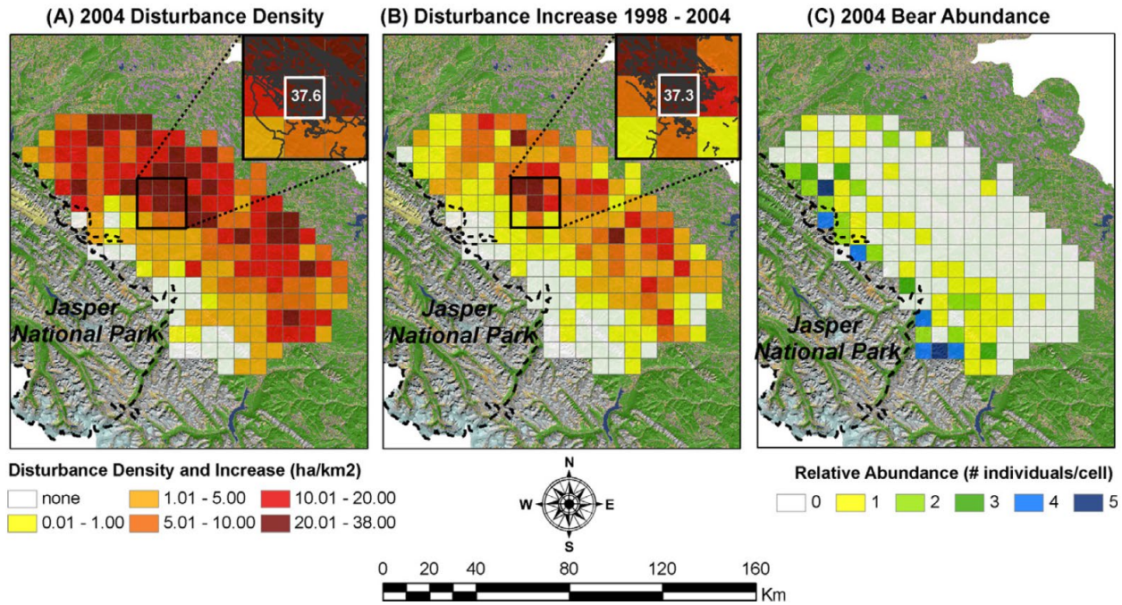
Figure 10. Distribution of (A) cumulative disturbance density existing in the study area at year 2004, and (B) the total increase in cumulative density between the years 1998 and 2004, and (C) the relative abundance of grizzly bears in the year 2004, based on repeated DNA-hair-sampling counts, across 178 landscape cells of the study area. Enlarged inserts show the underlying distribution of the actual cumulative disturbance features by 2004 (B) and of the new disturbance features gained between 1998 and 2004. Figure taken from Linke et al. 2013, p. 97.
