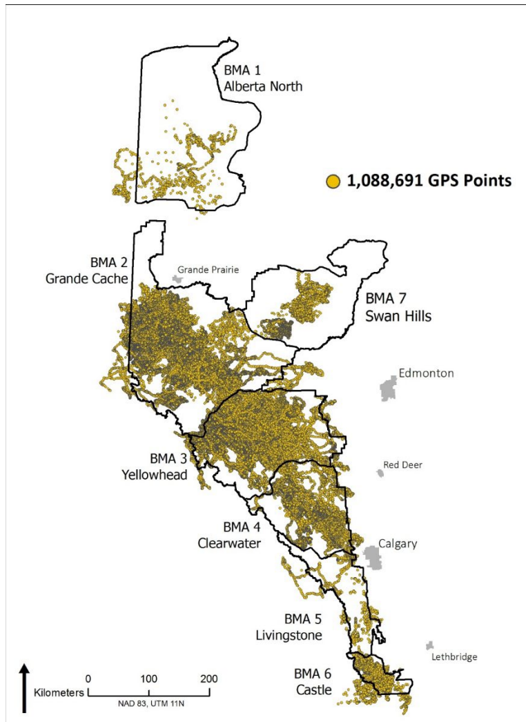
Figure 10. Grizzly bear telemetry data across all BMUs.
