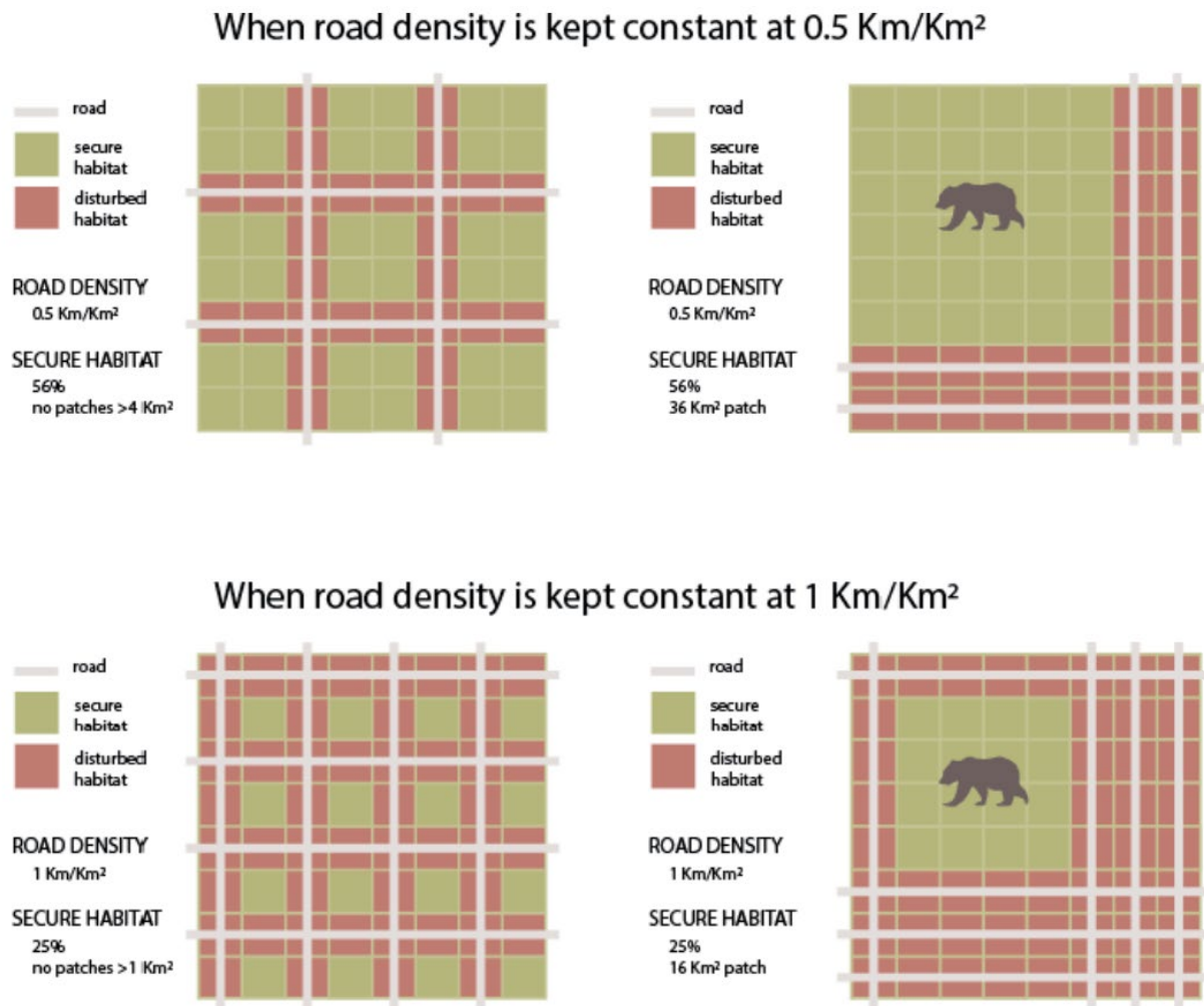
Figure 11. Schematic of the relationship between road density and the proportion of secure grizzly bear ( Ursus arctos ) habitat. Evenly spaced roads across a unit can result in small patches of secure habitat (i.e., areas >500 m from an open road) that require female bears to cross roads often during a day (panels on left). Managing road distribution to yield larger patches of secure habitat (panels on right), even at similar road densities, should benefit females and result in healthier grizzly bear populations. Figure from Proctor et al. 2020, p. 105.
