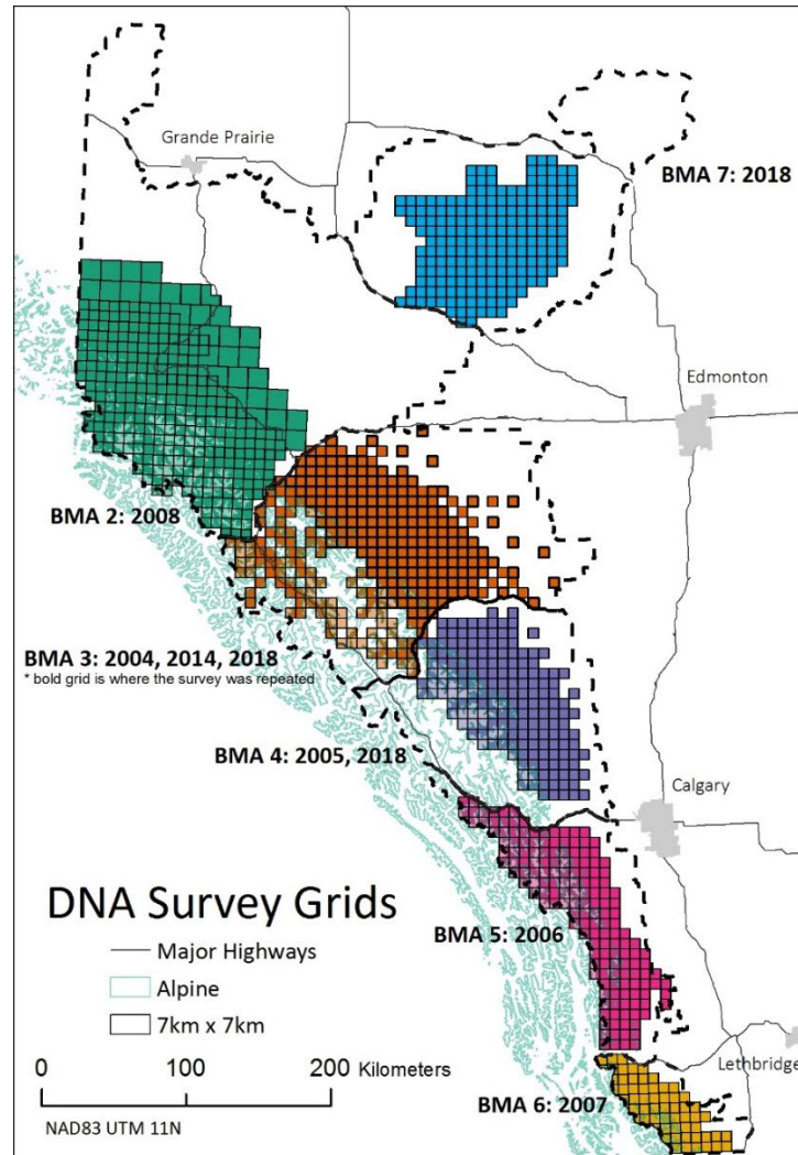
Figure 25. Survey grids used for DNA-based population inventories in all BMAs.
