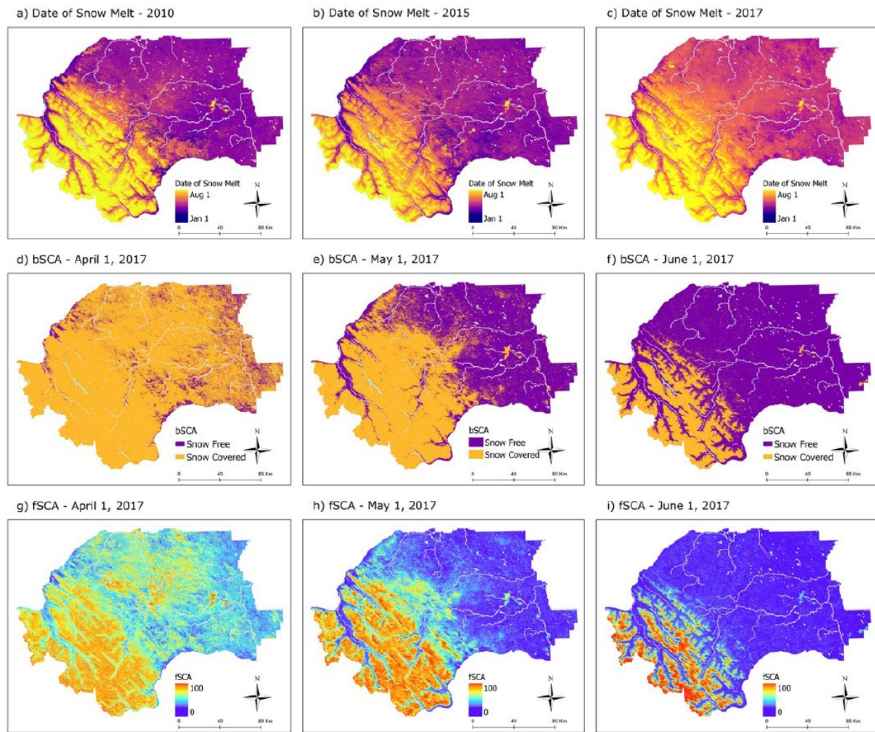
Figure 23. The three snow metrics derived from SNOWARP (Berman et al. 2018) at 30 m spatial resolution for years 2009-2017. a-c) Annual date of snow melt shown for spring 2010, 2015, and 2017. Days since snow melt (DSM) was produced by subtracting date of snow melt from the date associated with each grizzly bear telemetry location. d-f) daily binary snow covered area (bSCA) shown on April 1, May 1, and June 1, 2017. g-i) daily fractional snow covered area (fSCA) shown on April 1, May 1, and June 1, 2017. Figure from Berman et al. 2019, p. 121.
